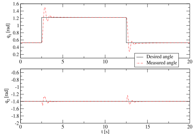
Fig. 3: System response to a step change in desired angle values (while using PID control).
